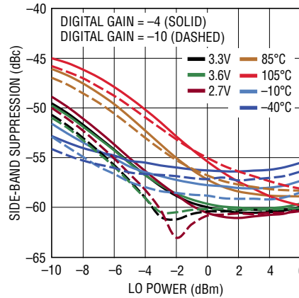
Side-Band Suppression vs LO Power at f_{LO} = 150MHz
